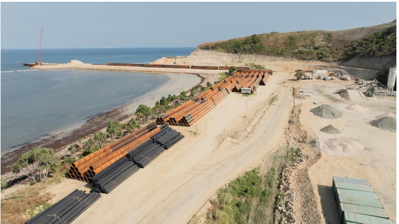
Image: 369 tubular piles delivered to site for the Wharf Phase 3 extension
